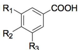
Hydroxybenzoic acid
